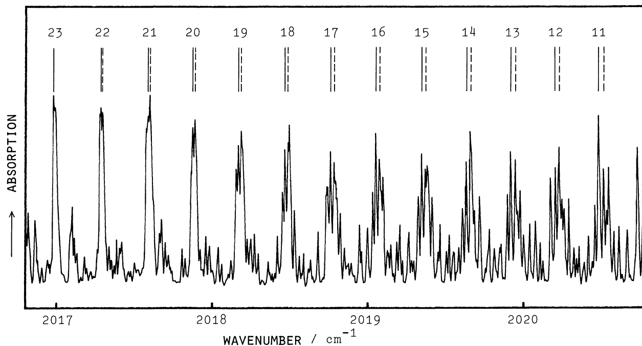
Fig. 1. Part of the high-resolution spectrum of OCS e near 2019 \text{ cm}^{-1} . Numbers correspond to J values for the J-1+J ( 10^0_0-00^0_0 ) transitions. Solid lines: ^{16}\text{O}^{12}\text{C}^{80}\text{Se} . Broken lines: ^{16}\text{O}^{12}\text{C}^{78}\text{Se} .
